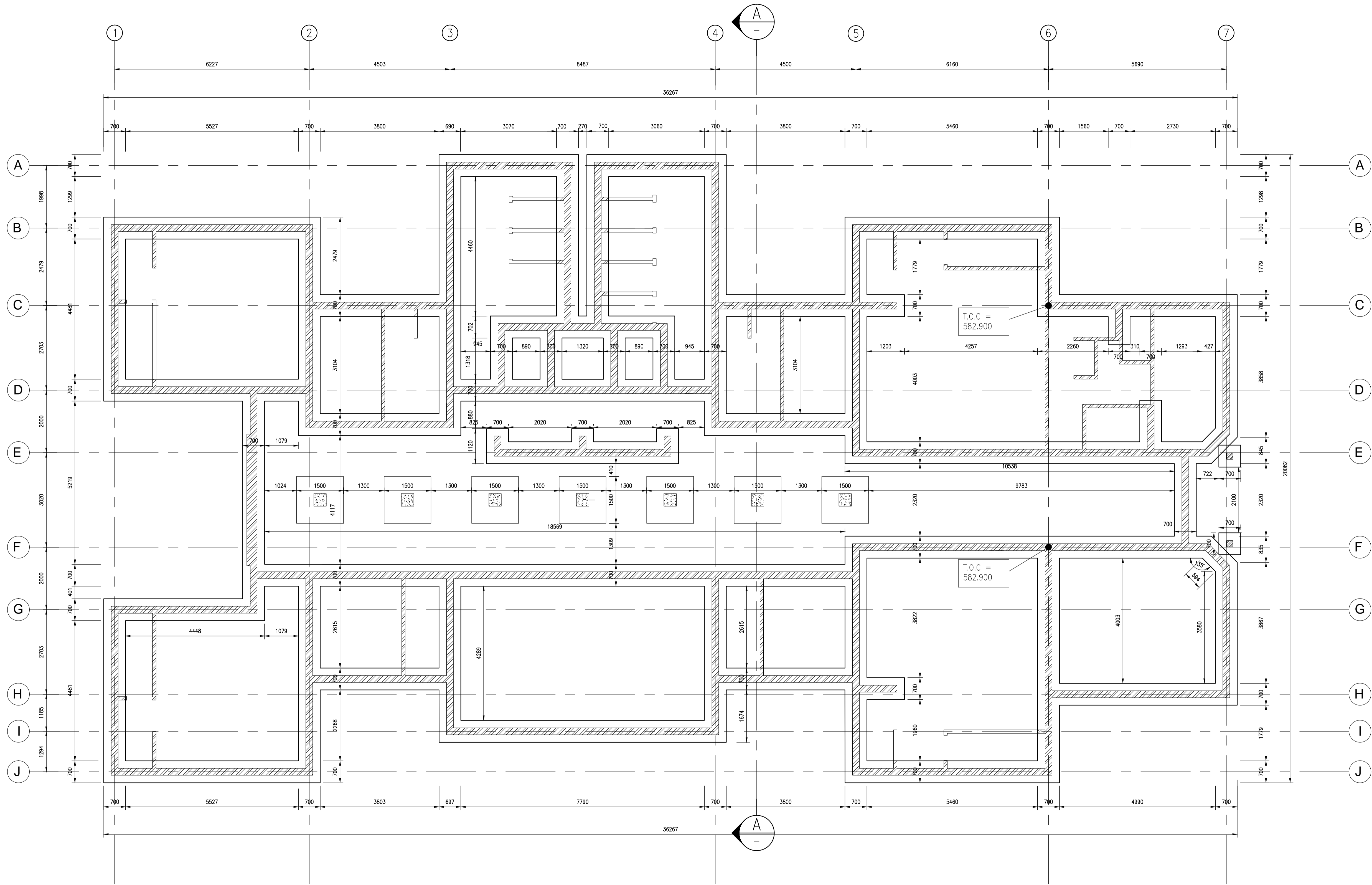
FOUNDATION LAYOUT SCALE 1:50
